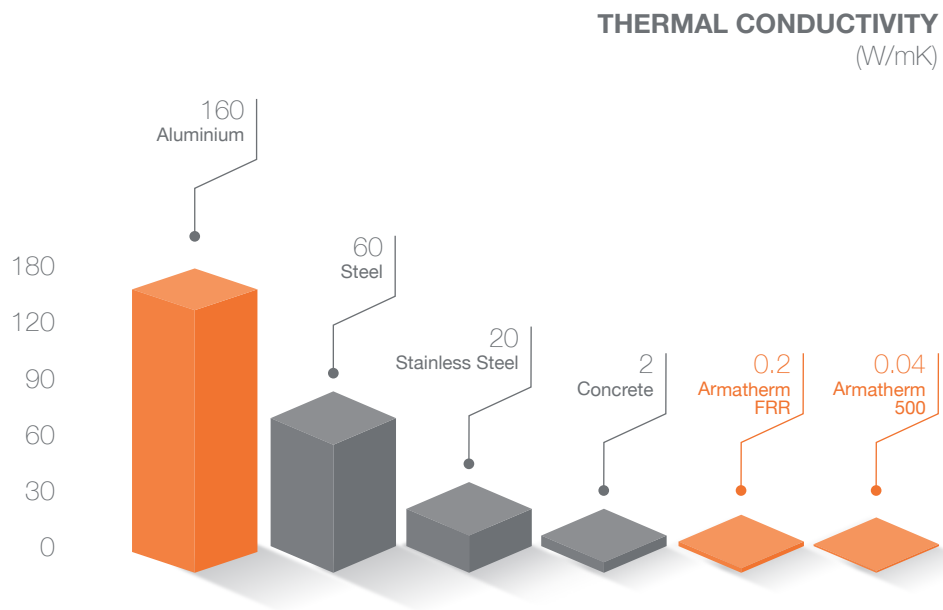
Thermal conductivity values of Armatherm™ structural thermal break materials as compared to standard building materials.
