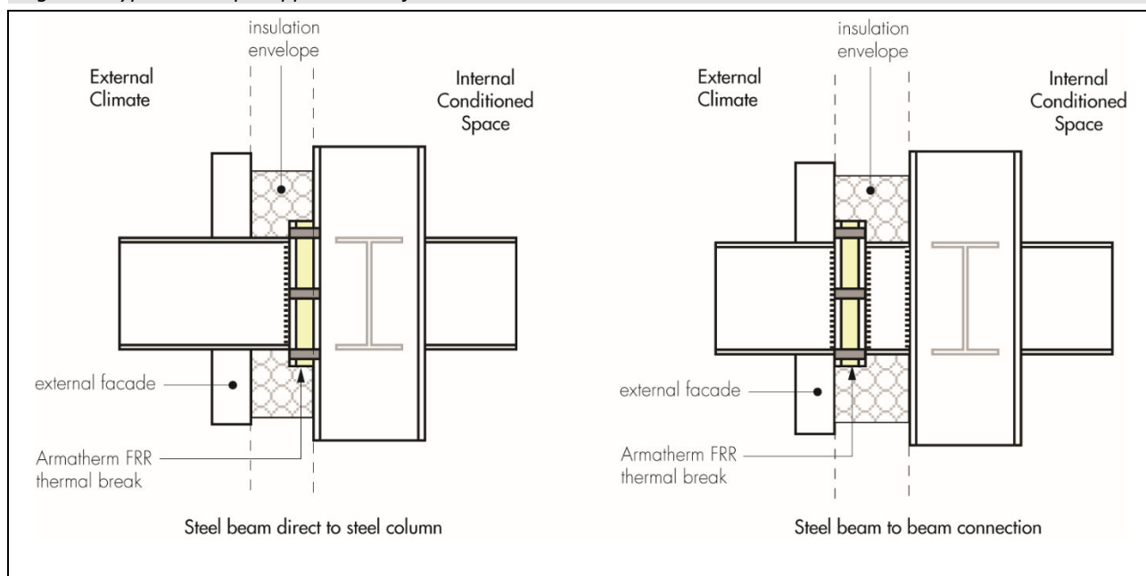
Figure 2 Typical example applications of Armatherm FRR at external walls
